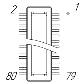
DF40 80 pin header bottom view
